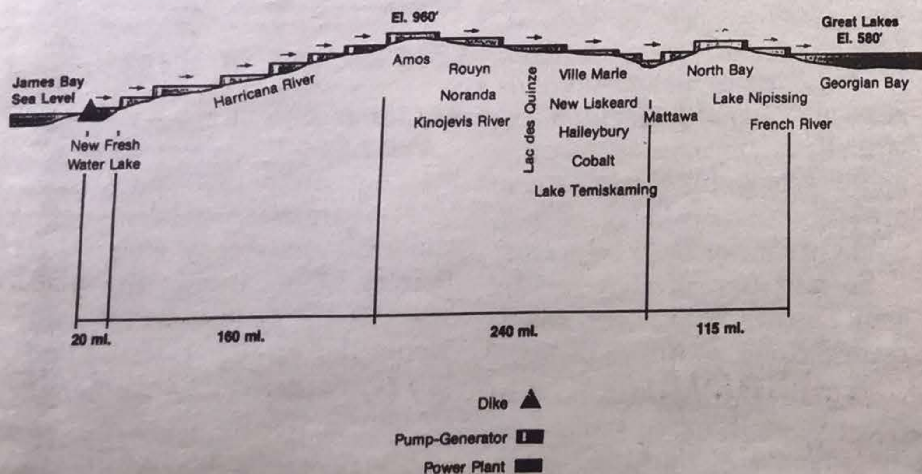
Figure 9-7 Recycling Water from James Bay to the Great Lakes
